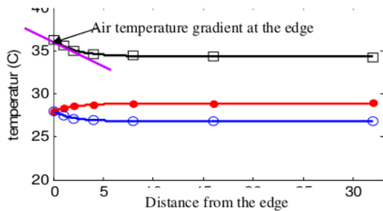
Mathematic (Figure-1, t Figure 1. Spatial changes of air temperature at 07.00 a.m. (blue), 13.00 p.m. (black) and 23.00 p.m. (red) location, to 23:00 hours
